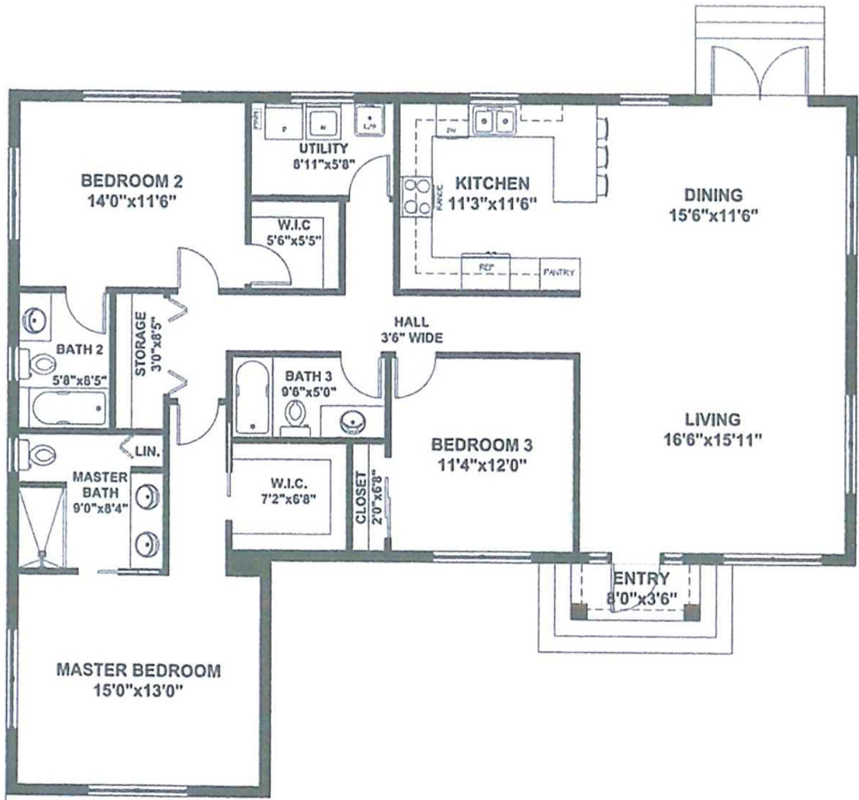
FLOOR PLAN - MBF
